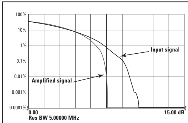
Figure 18: Compression effects displayed by CCDF curves.
